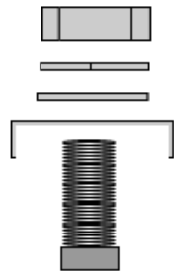
M10 Nut & Bolt Assembly With Plain Washer, Spring Washer & Plate
